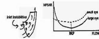
Fig. 7 Impeller Eye vs. NPSH_R [16]
