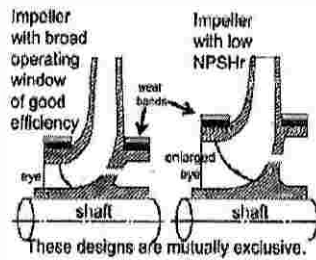
Fig. 9 Ns vs High Efficiency
