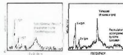
Fig. 15 Cavitation & Recirculation [22]
