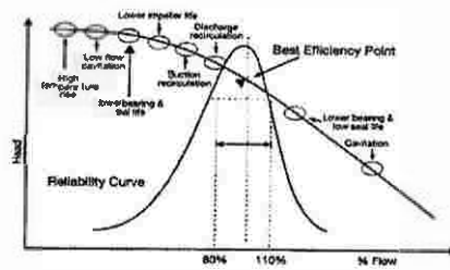
Fig. 4 Best Efficiency Point [15]
