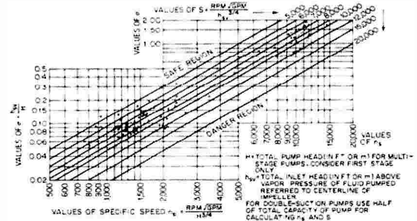
Fig. 13 Cavitation Regions [20]
