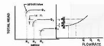
Fig. 14 NPSH_R Curve [21]
