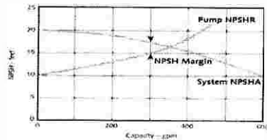
Fig. 3 NPSH Margin Ratio [13]
