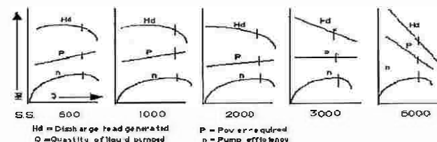
Fig. 2 Head vs. Specific Speed [10]
