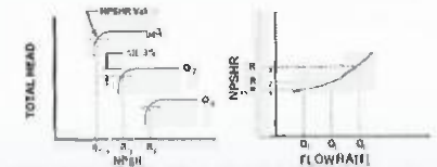
Fig. 14 NPSH_R Curve [21]
