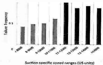
Fig. 11 Failure Frequency vs. Suction Specific Speed [24]
