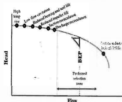
Fig. 1 Head vs. Capacity Curve [25]
