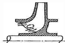
Fig. 5 Suction Recirculation [1]
