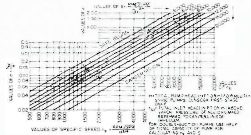
Fig. 13 Cavitation Regions [20]
