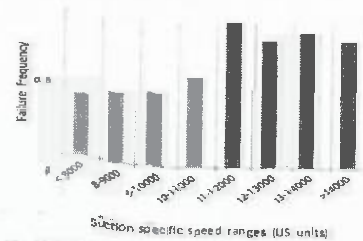
Fig. 11 Failure Frequency vs. Suction Specific Speed [24]
