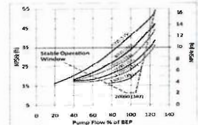
Fig. 8 Window Margin [24]
